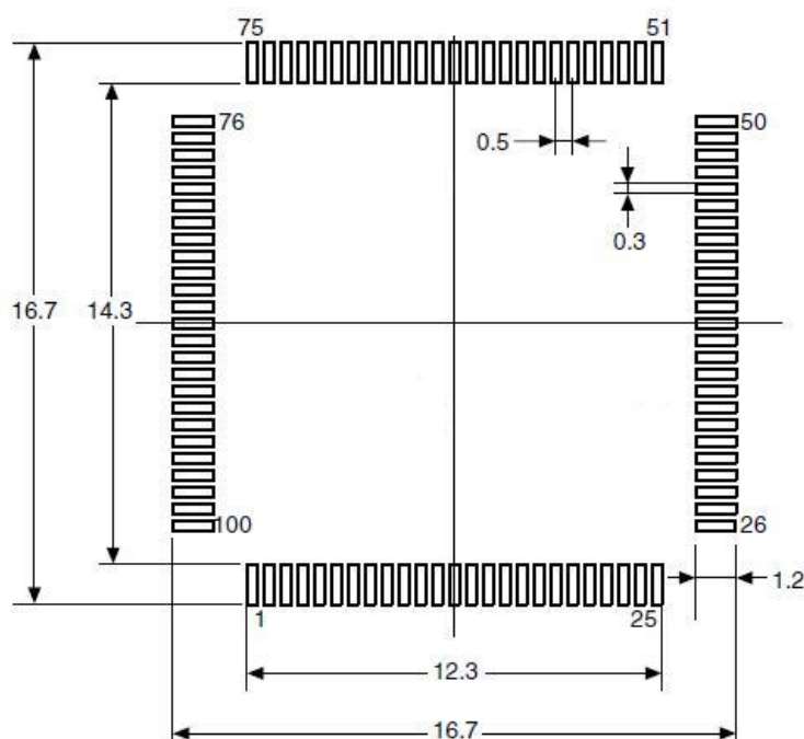
Figure 17 LQFP100 - 100 Pins, 14 x 14mm Welding Layout Recommendations
