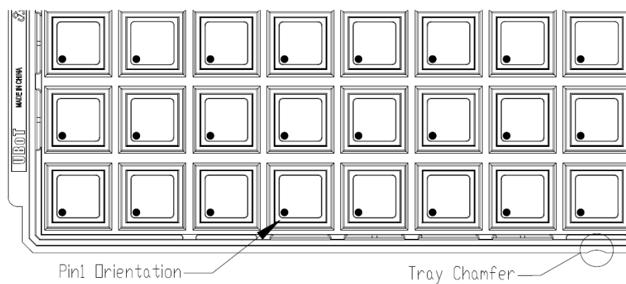
Figure 19 Tray Packaging Diagram
